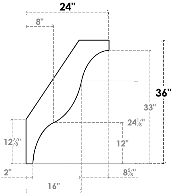
SIDE PROFILE
